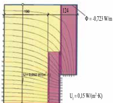
Trasmittanza termica U_f = 0,15 \text{ W/m}^2\text{K}
