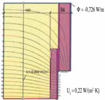
Trasmittanza termica U_f = 0,22 \text{ W/m}^2\text{K}
